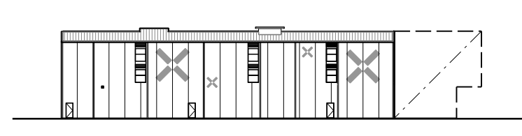
03 EAST ELEVATION 1:250
