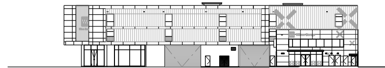
02 WEST ELEVATION 1:250
