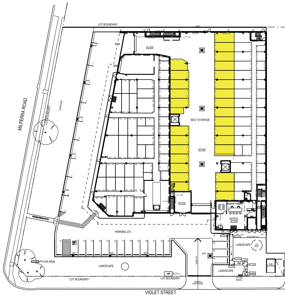
01 GROUND FLOOR PLAN 1:250
